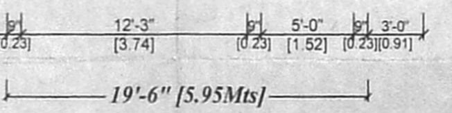
Terrace Floor Plan
